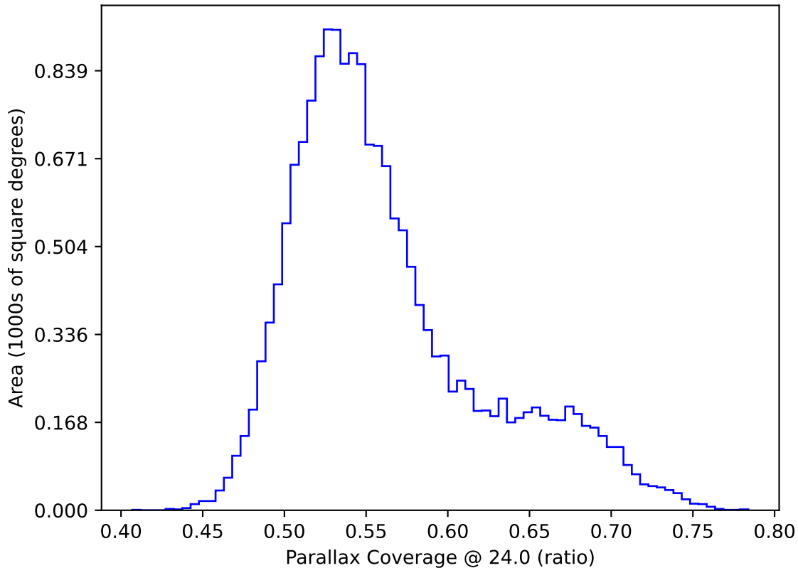
weather_cloudso0v3.4_10yrs WFD: Parallax Coverage @ 24.0
