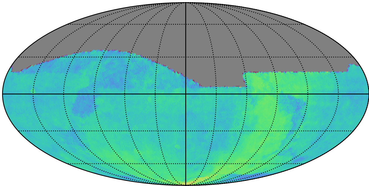
weather_cloudso0v3.4_10yrs All sky: Parallax Coverage @ 24.0
