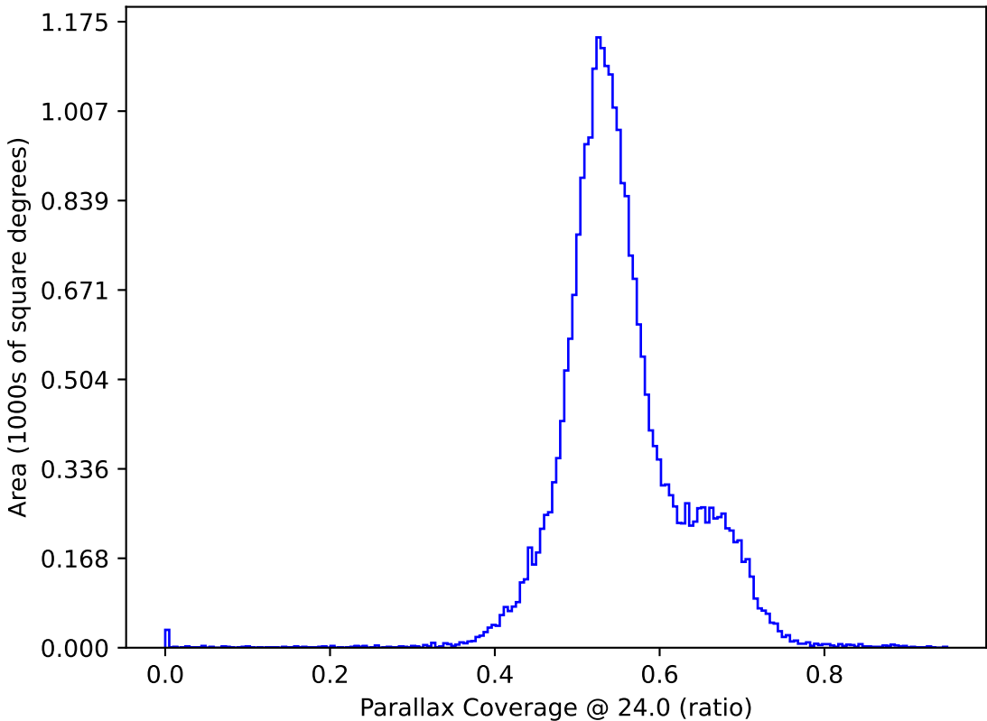
weather_cloudso0v3.4_10yrs All sky: Parallax Coverage @ 24.0
