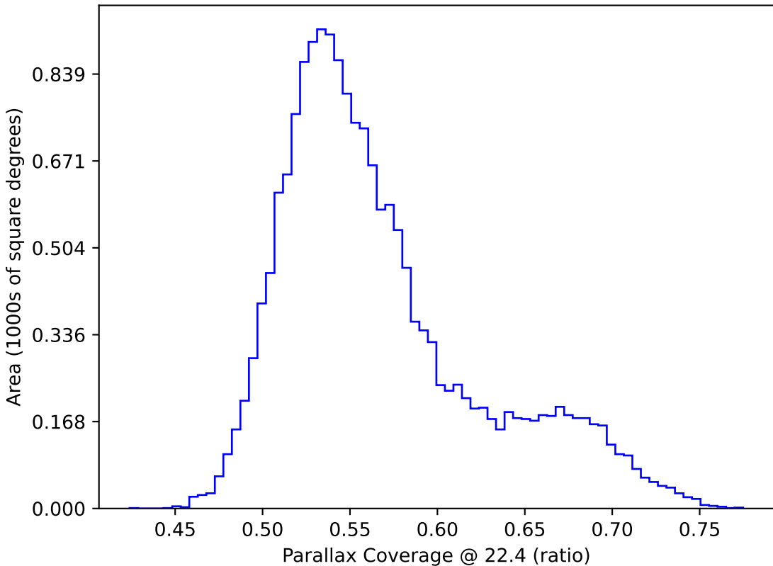
weather_cloudso0v3.4_10yrs WFD: Parallax Coverage @ 22.4
