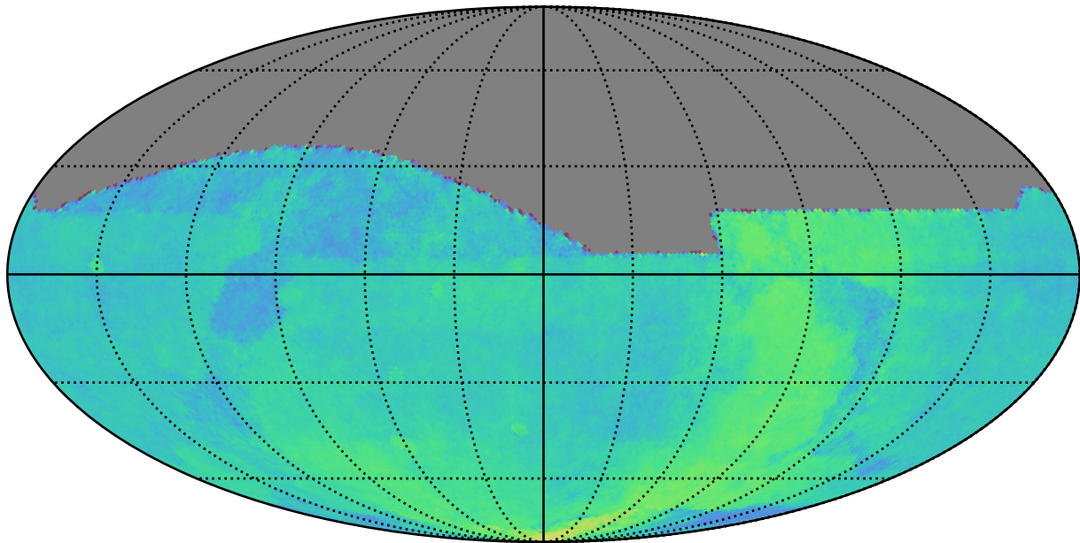
weather_cloudso0v3.4_10yrs All sky: Parallax Coverage @ 22.4
