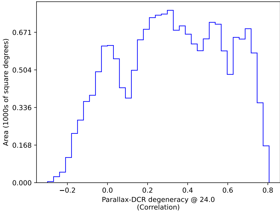
weather_cloudso0v3.4_10yrs WFD: Parallax-DCR degeneracy @ 24.0
