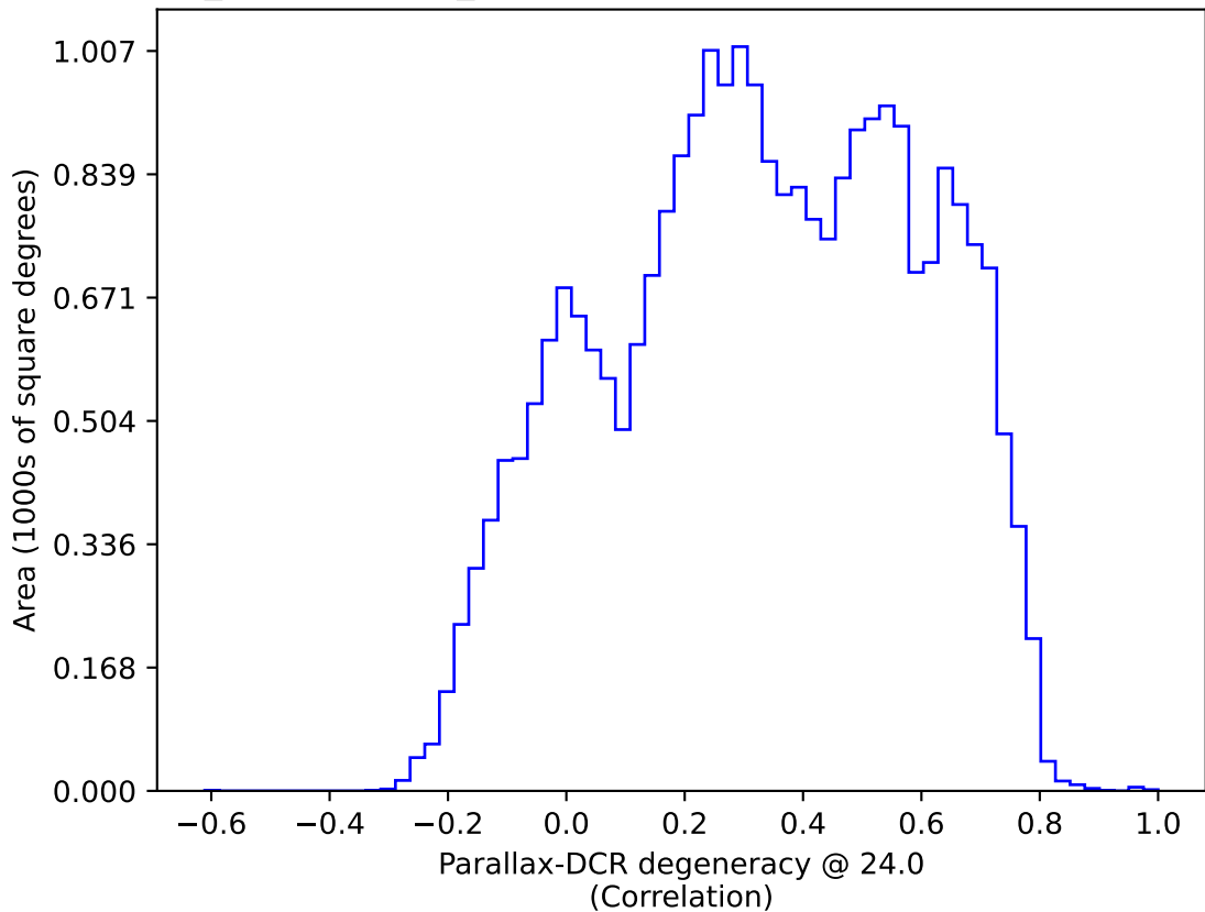
weather_cloudso0v3.4_10yrs All sky: Parallax-DCR degeneracy @ 24.0
