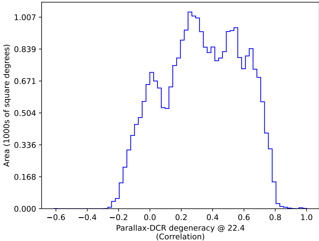
weather_cloudso0v3.4_10yrs All sky: Parallax-DCR degeneracy @ 22.4
