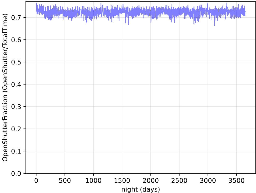
weather_cloudso0v3.4_10yrs Per night: OpenShutterFraction
