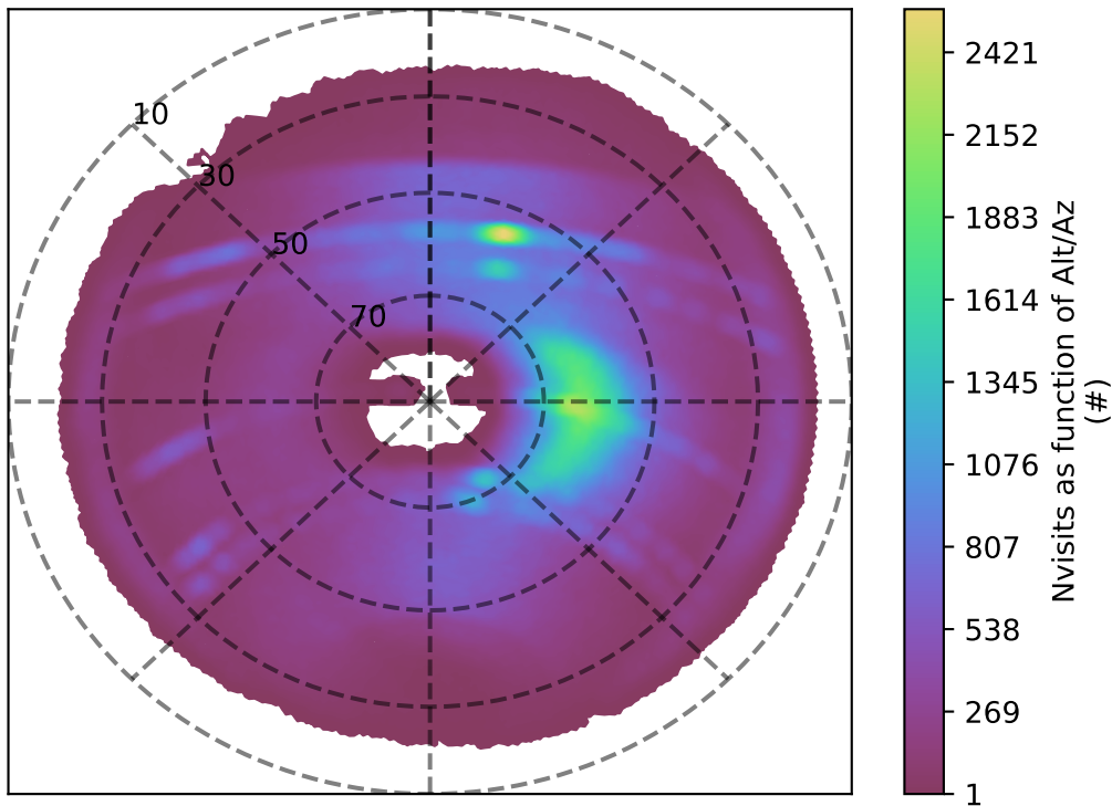
weather_cloudso0v3.4_10yrs z band: Nvisits as function of Alt/Az
