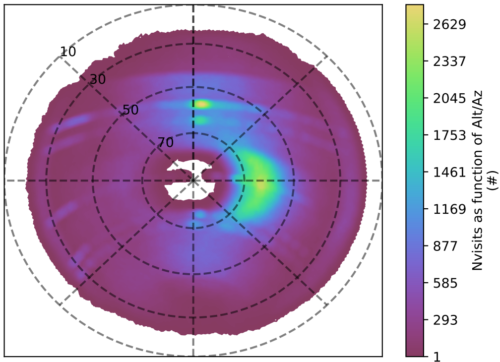
weather_cloudso0v3.4_10yrs i band: Nvisits as function of Alt/Az
