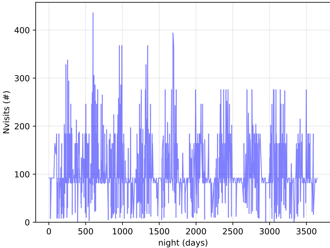
weather_cloudso0v3.4_10yrs DDF: Nvisits
