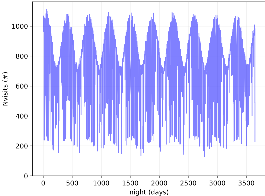
weather_cloudso0v3.4_10yrs All visits: Nvisits
