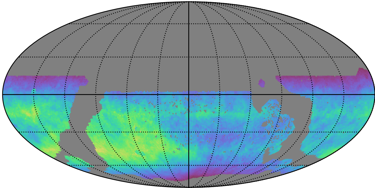
weather_cloudso0v3.4_10yrs WFD z band: Normalized Teff
