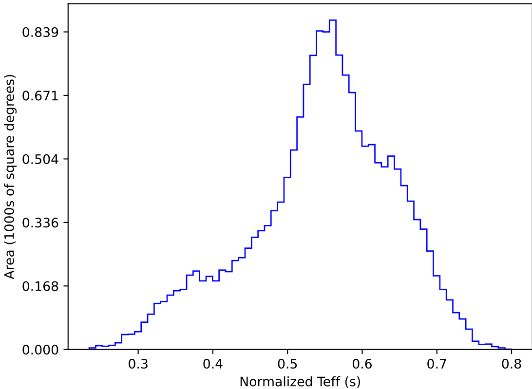
weather_cloudso0v3.4_10yrs WFD y band: Normalized Teff
