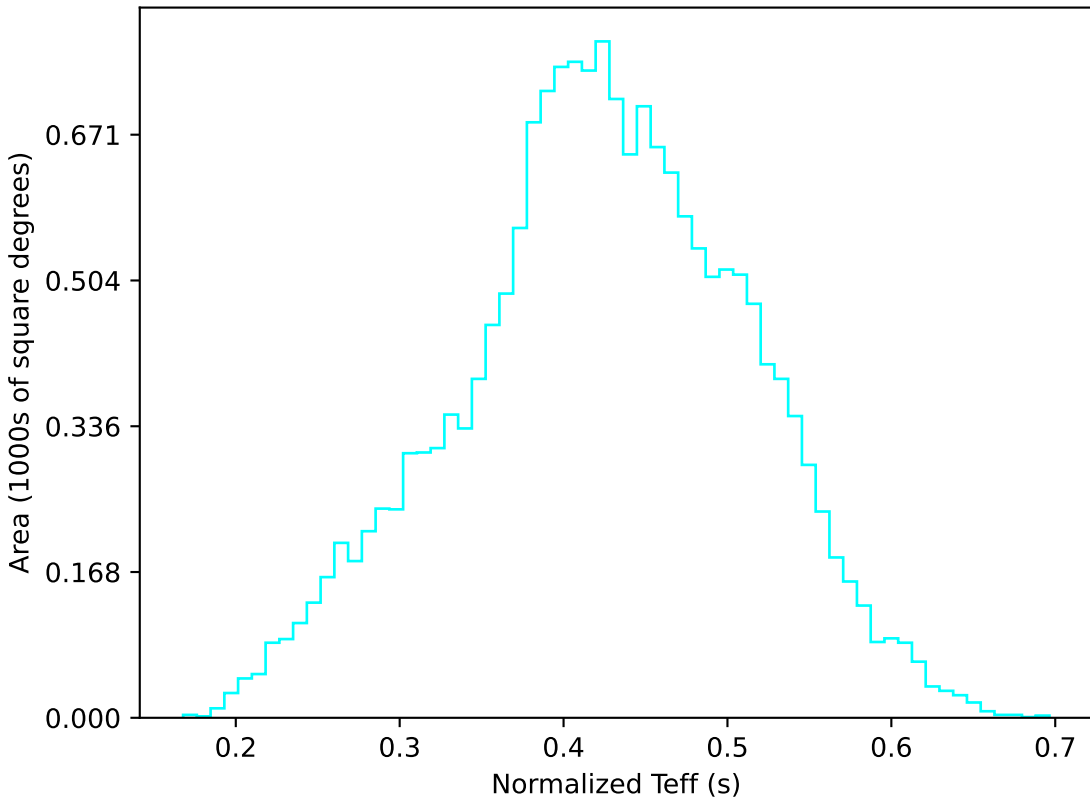
weather_cloudso0v3.4_10yrs WFD u band: Normalized Teff
