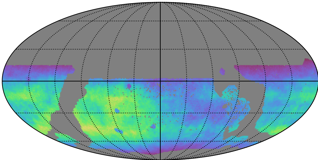
weather_cloudso0v3.4_10yrs WFD r band: Normalized Teff
