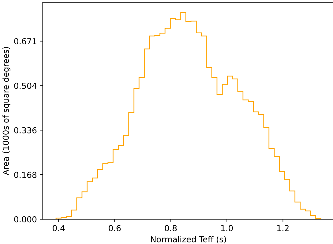
weather_cloudso0v3.4_10yrs WFD r band: Normalized Teff
