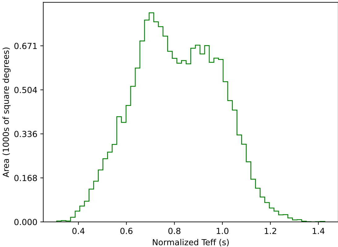
weather_cloudso0v3.4_10yrs WFD g band: Normalized Teff
