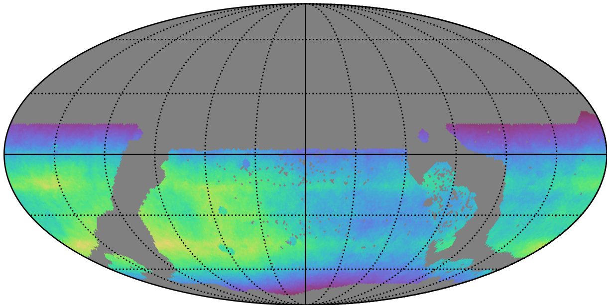
weather_cloudso0v3.4_10yrs WFD all bands: Normalized Teff
