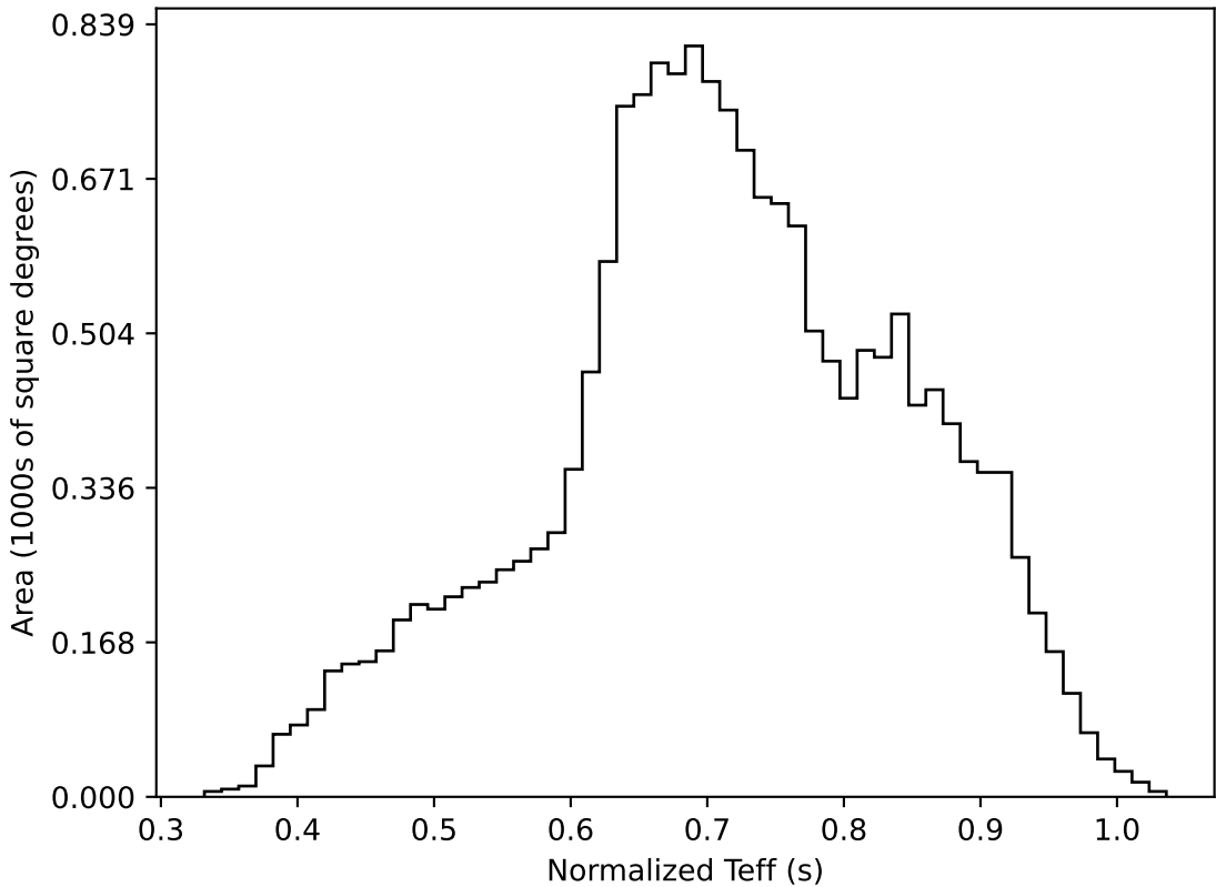
weather_cloudso0v3.4_10yrs WFD all bands: Normalized Teff
