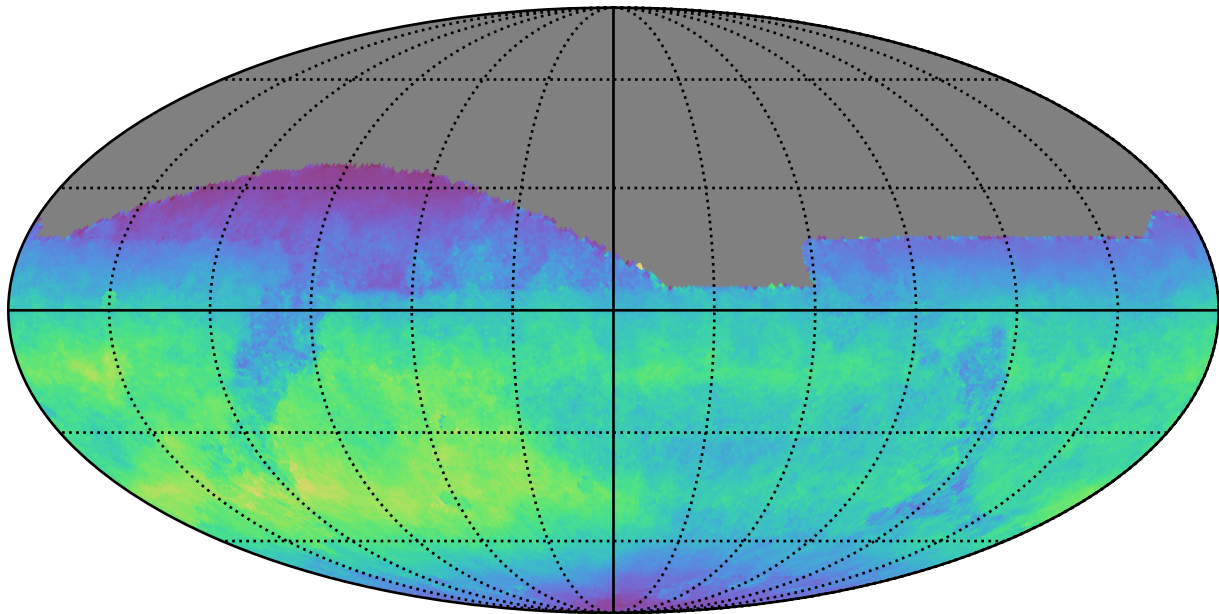
weather_cloudso0v3.4_10yrs All sky z band: Normalized Teff
