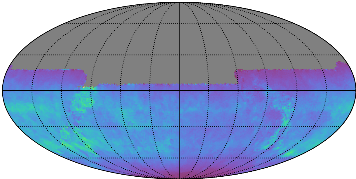
weather_cloudso0v3.4_10yrs All sky u band: Normalized Teff
