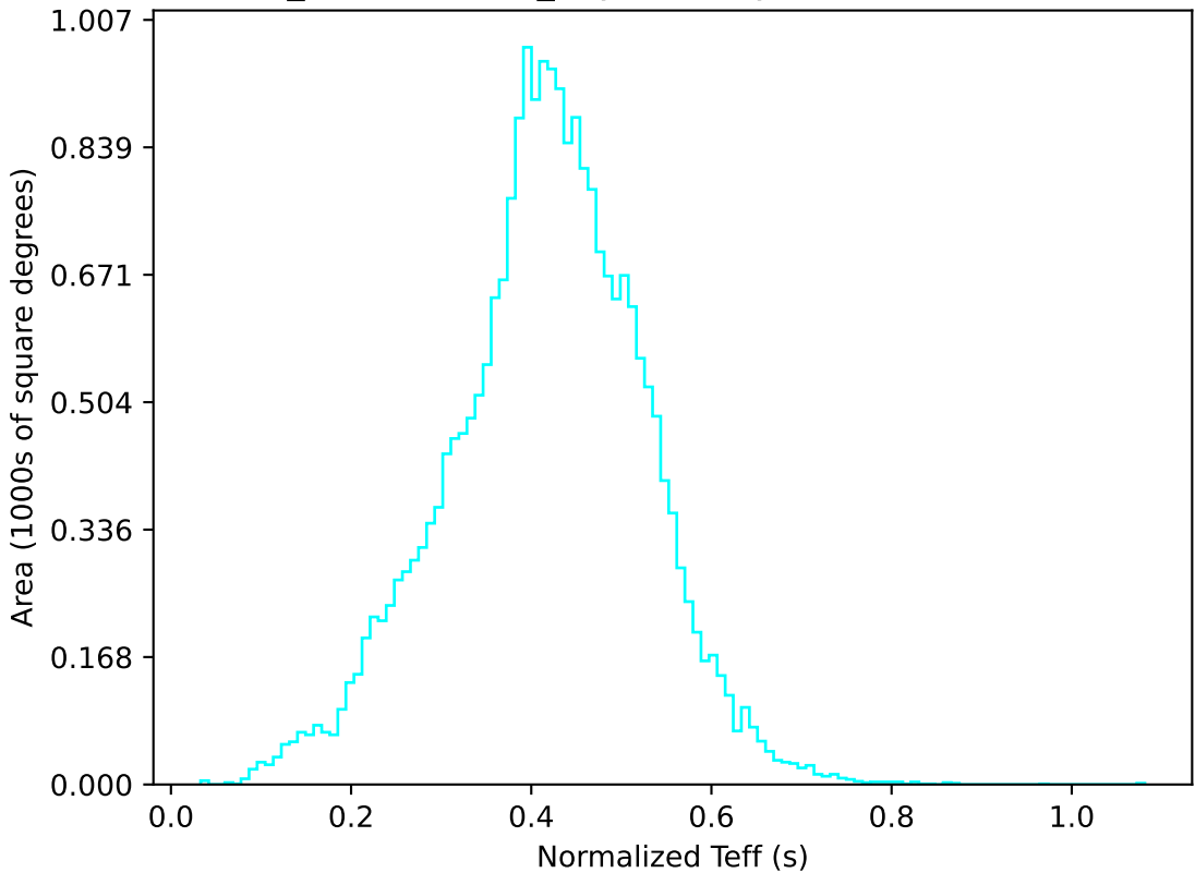
weather_cloudso0v3.4_10yrs All sky u band: Normalized Teff
