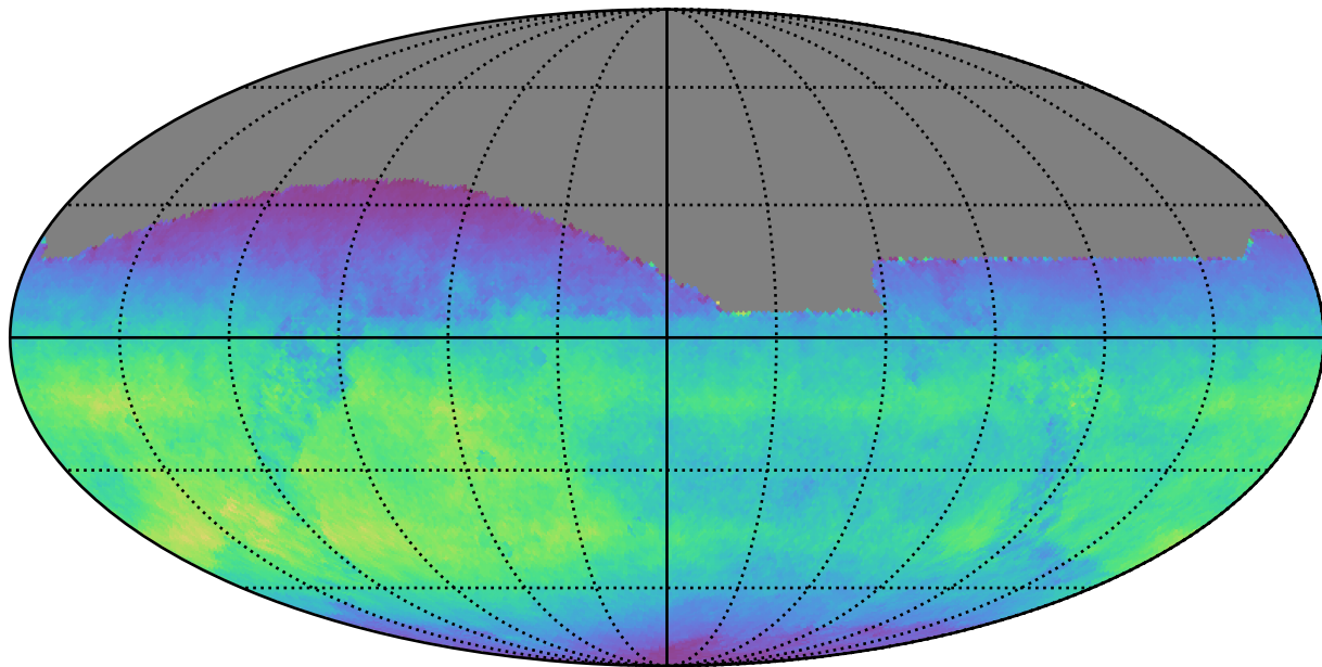
weather_cloudso0v3.4_10yrs All sky i band: Normalized Teff
