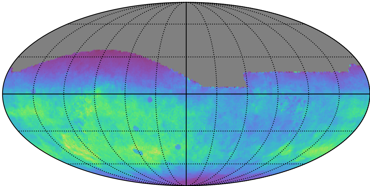
weather_cloudso0v3.4_10yrs All sky g band: Normalized Teff
