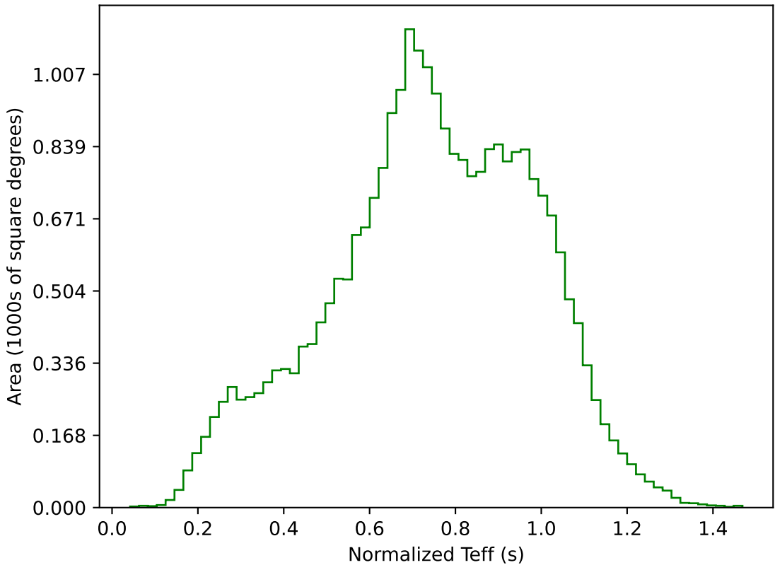
weather_cloudso0v3.4_10yrs All sky g band: Normalized Teff
