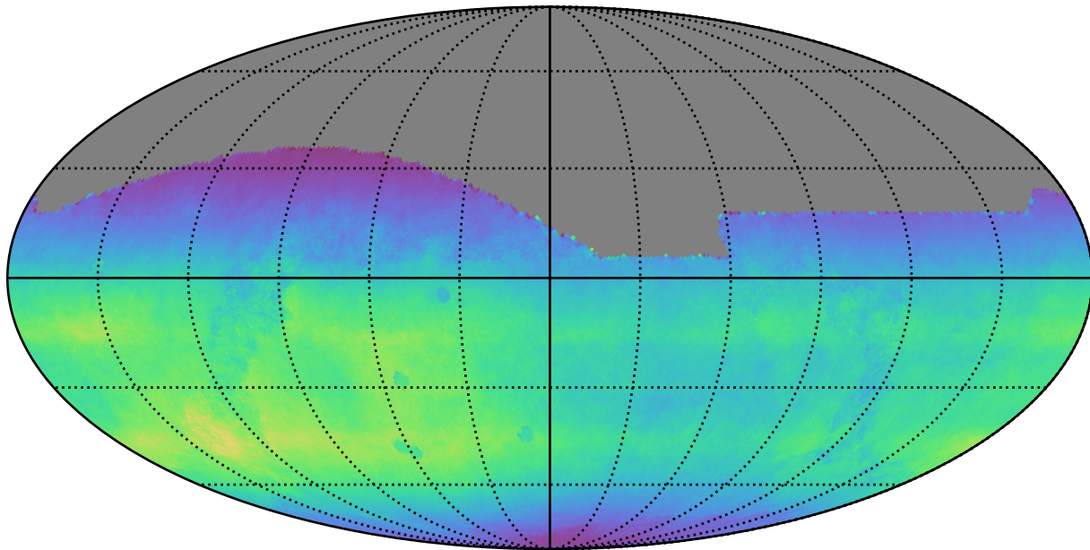
weather_cloudso0v3.4_10yrs All sky all bands: Normalized Teff
