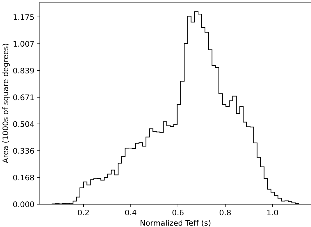
weather_cloudso0v3.4_10yrs All sky all bands: Normalized Teff
