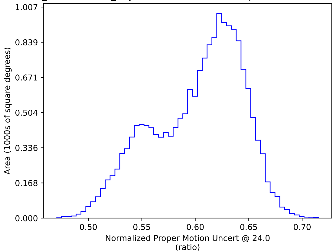
weather_cloudso0v3.4_10yrs WFD: Normalized Proper Motion Uncert @ 24.0
