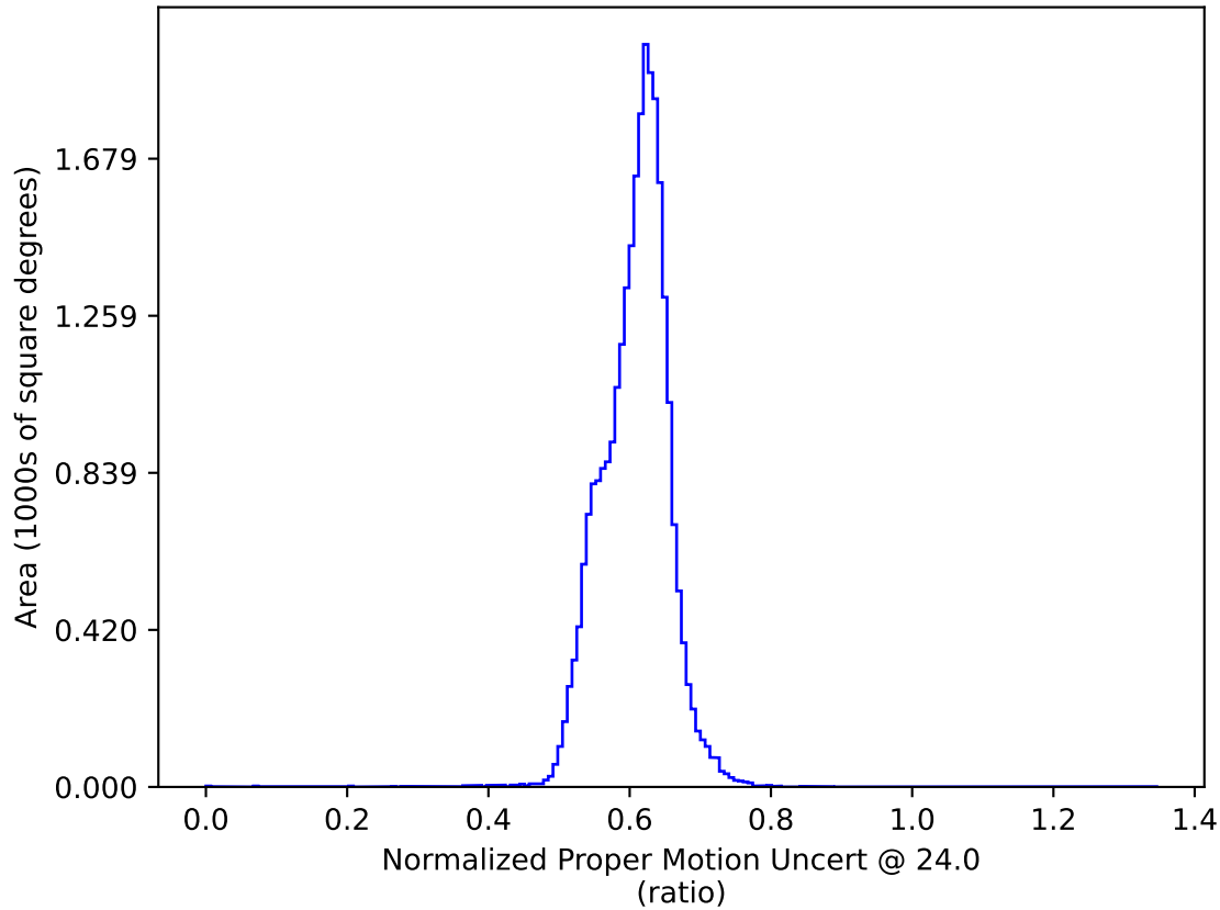
weather_cloudso0v3.4_10yrs All sky: Normalized Proper Motion Uncert @ 24.0
