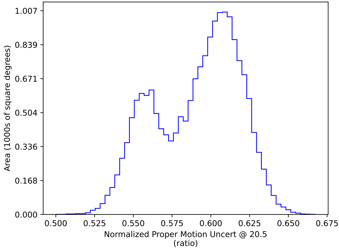
weather_cloudso0v3.4_10yrs WFD: Normalized Proper Motion Uncert @ 20.5
