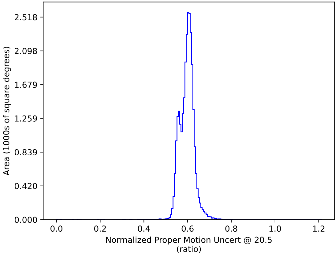
weather_cloudso0v3.4_10yrs All sky: Normalized Proper Motion Uncert @ 20.5
