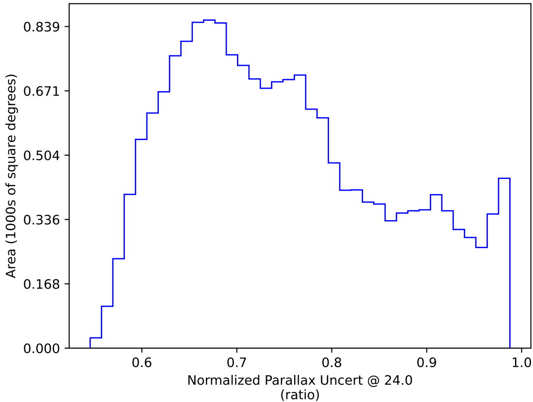
weather_cloudso0v3.4_10yrs WFD: Normalized Parallax Uncert @ 24.0
