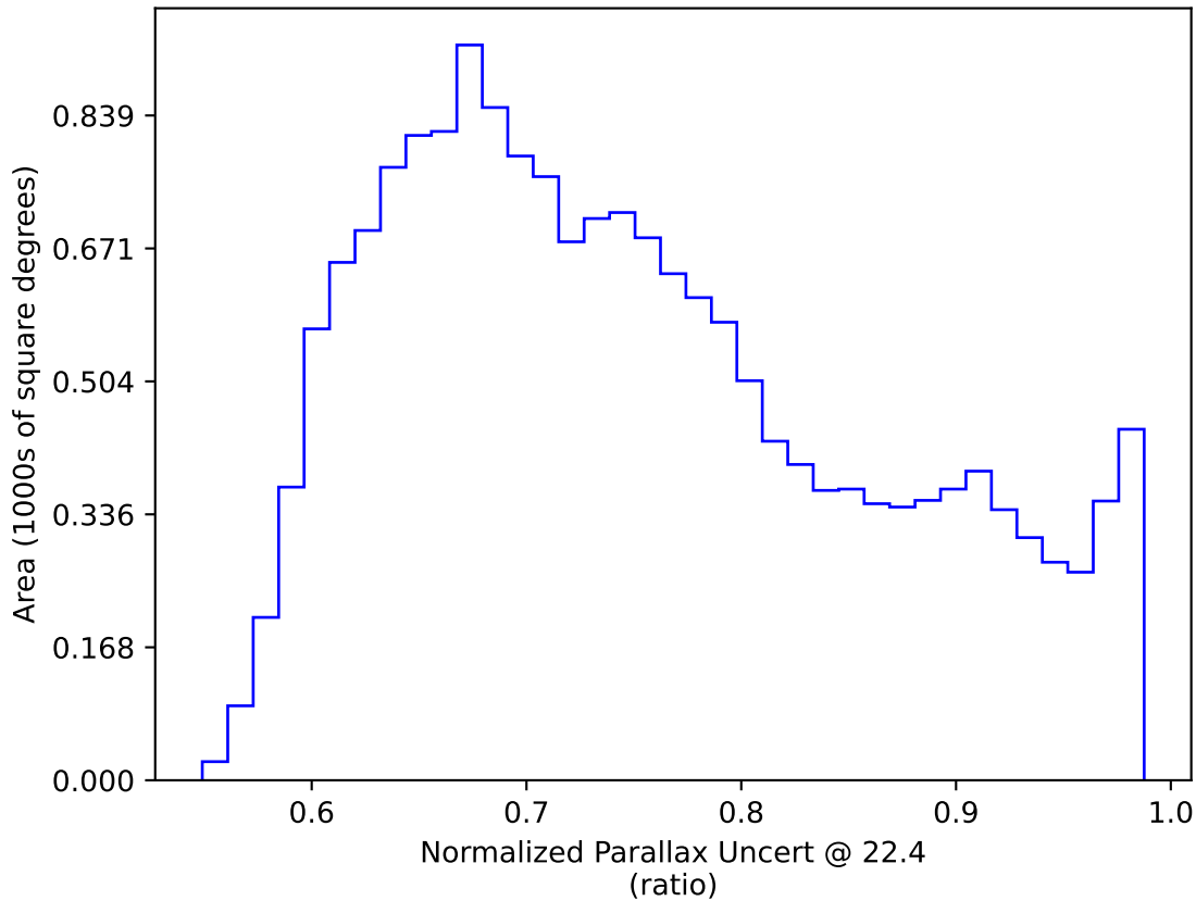
weather_cloudso0v3.4_10yrs WFD: Normalized Parallax Uncert @ 22.4
