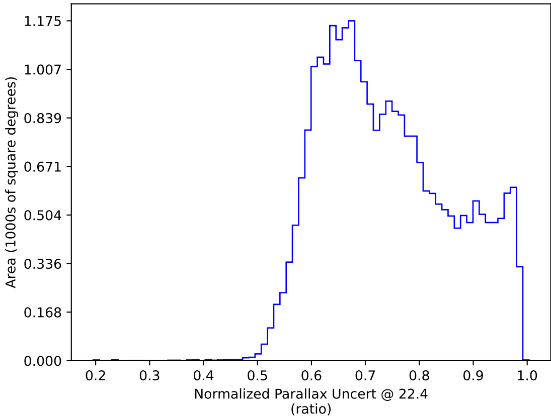
weather_cloudso0v3.4_10yrs All sky: Normalized Parallax Uncert @ 22.4
