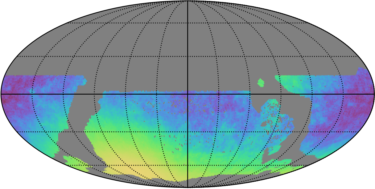
weather_cloudso0v3.4_10yrs WFD y band only: Normalized Parallax Uncert @ 21.3
