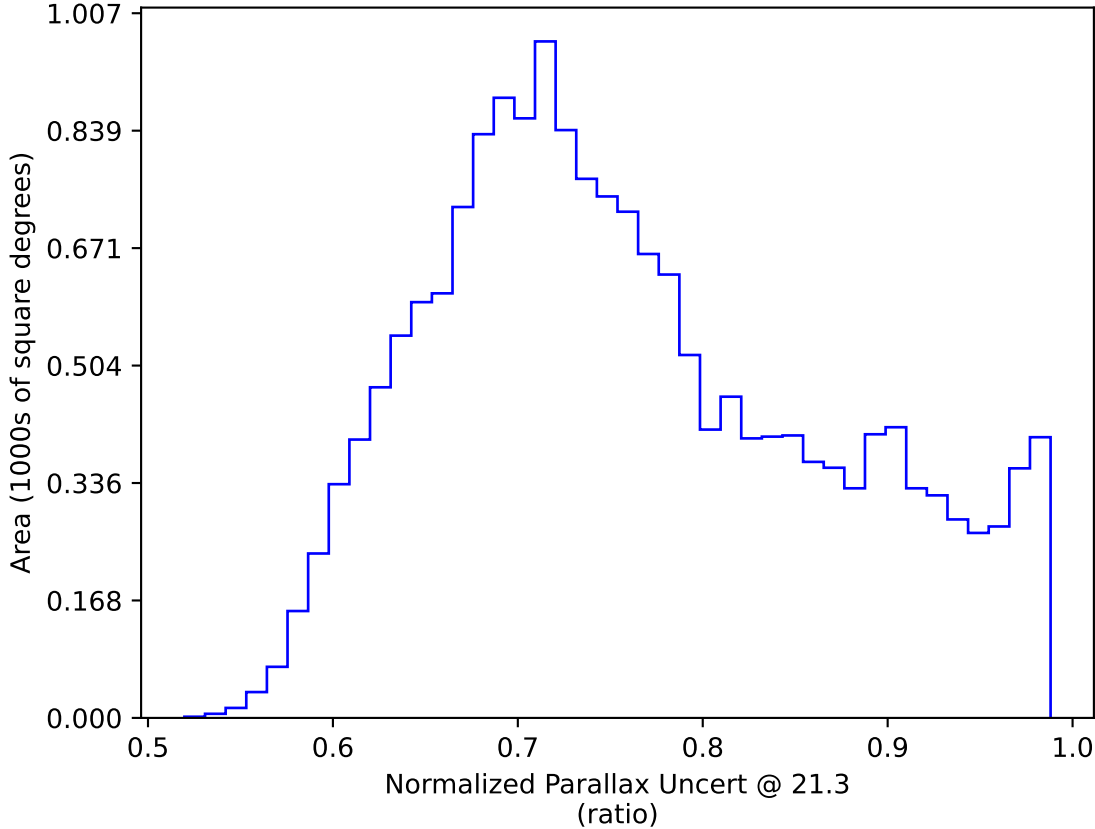
weather_cloudso0v3.4_10yrs WFD y band only: Normalized Parallax Uncert @ 21.3
