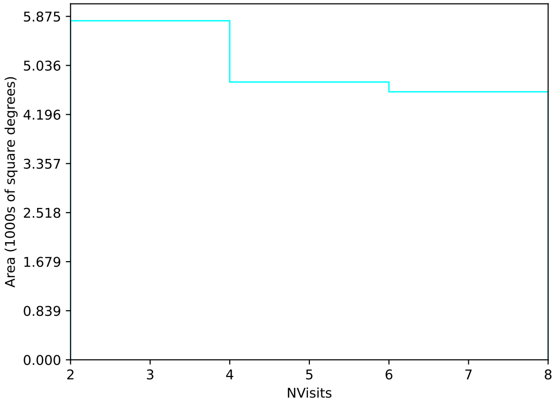
weather_cloudso0v3.4_10yrs Yr 3-4 u band: NVisits
