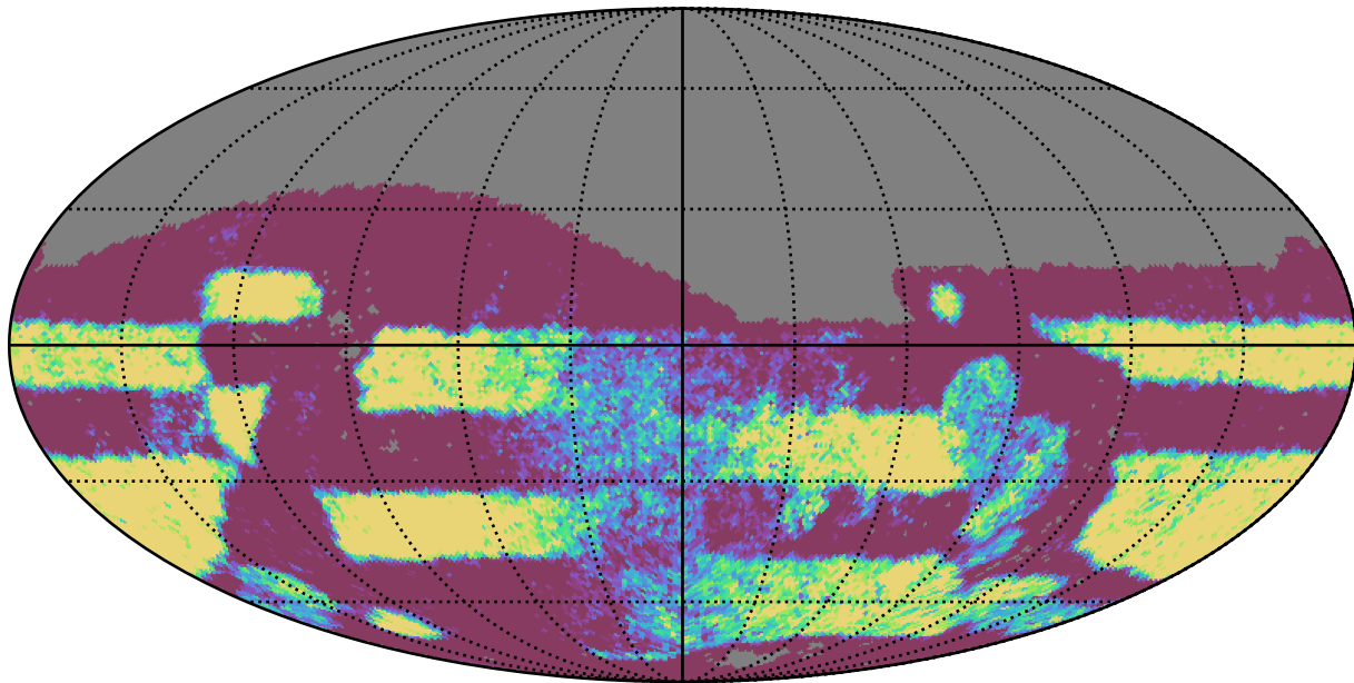
weather_cloudso0v3.4_10yrs Yr 3-4 r band: NVisits
