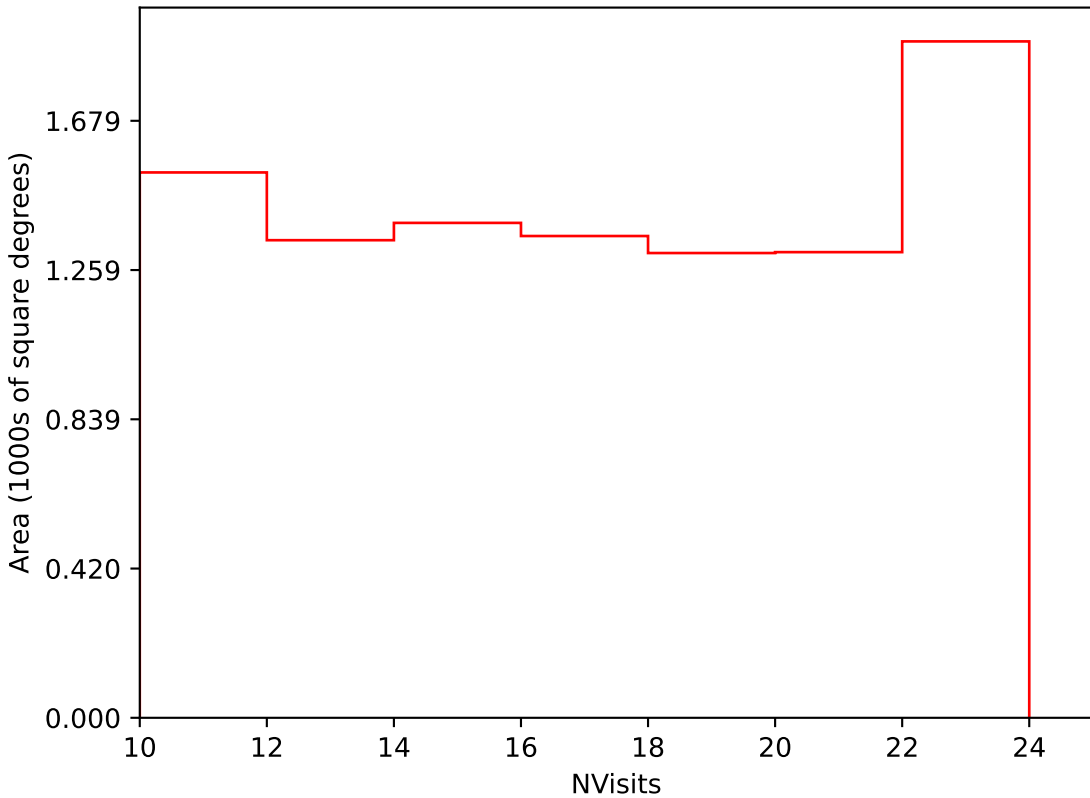
weather_cloudso0v3.4_10yrs Yr 3-4 i band: NVisits
