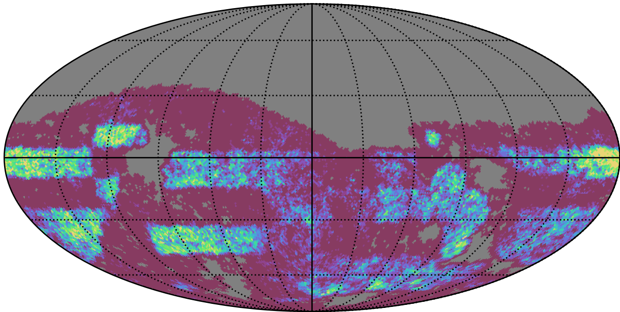
weather_cloudso0v3.4_10yrs Yr 3-4 g band: NVisits
