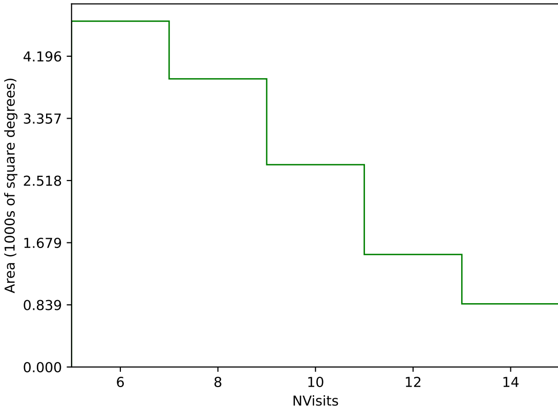
weather_cloudso0v3.4_10yrs Yr 3-4 g band: NVisits
