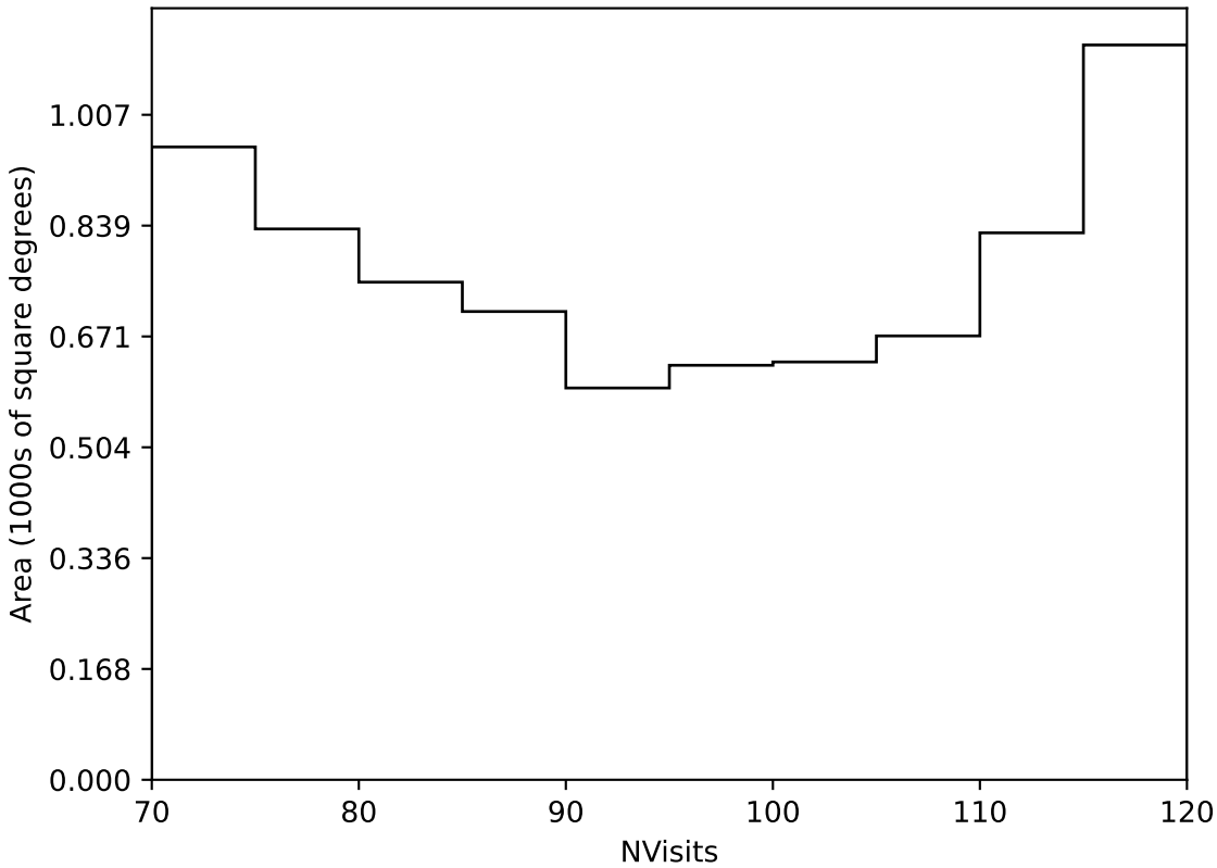
weather_cloudso0v3.4_10yrs Yr 3-4 all bands: NVisits
