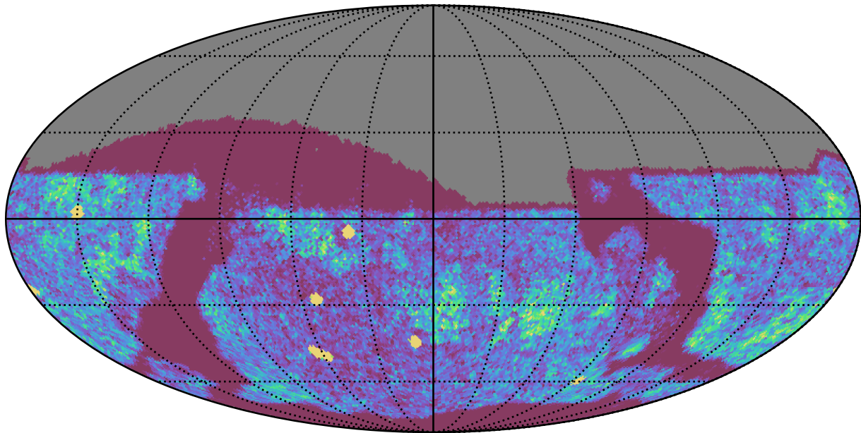
weather_cloudso0v3.4_10yrs Yr 1 z band: NVisits
