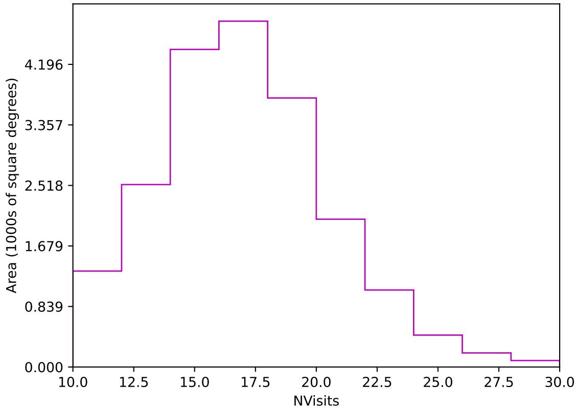
weather_cloudso0v3.4_10yrs Yr 1 z band: NVisits
