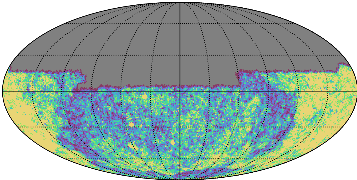
weather_cloudso0v3.4_10yrs Yr 1 u band: NVisits
