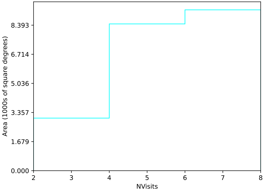
weather_cloudso0v3.4_10yrs Yr 1 u band: NVisits
