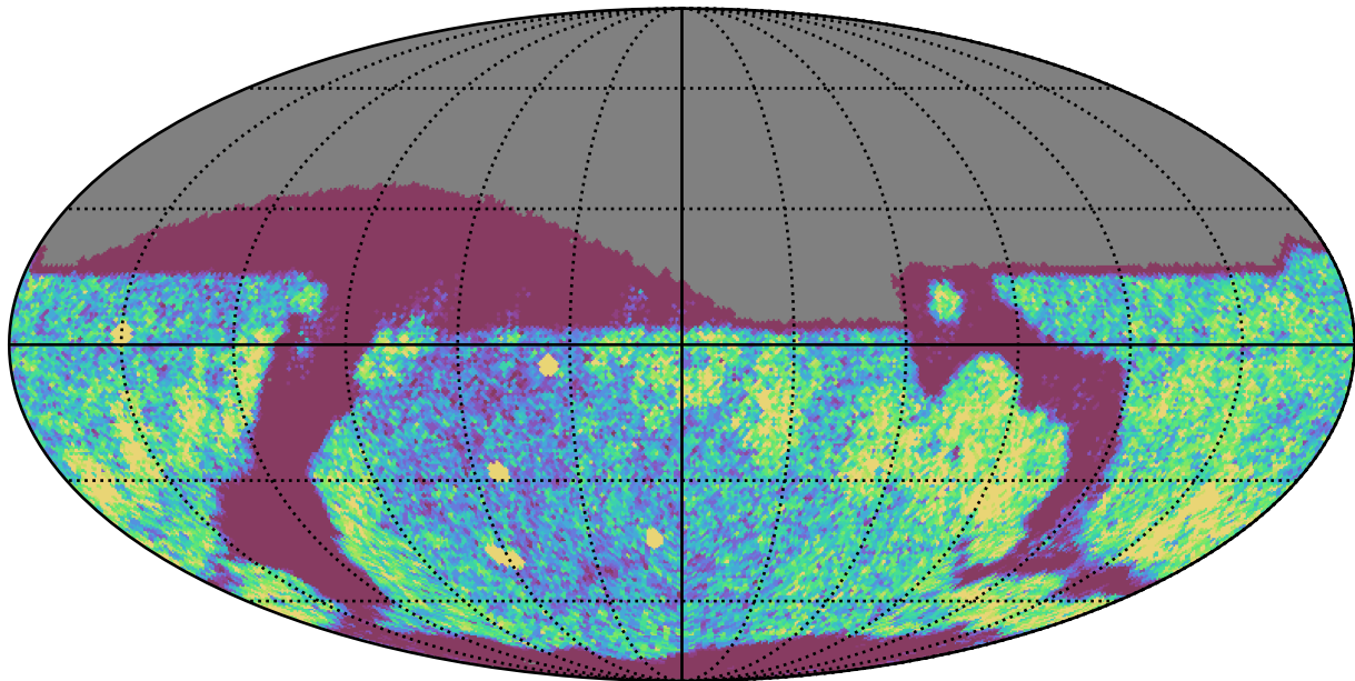
weather_cloudso0v3.4_10yrs Yr 1 r band: NVisits
