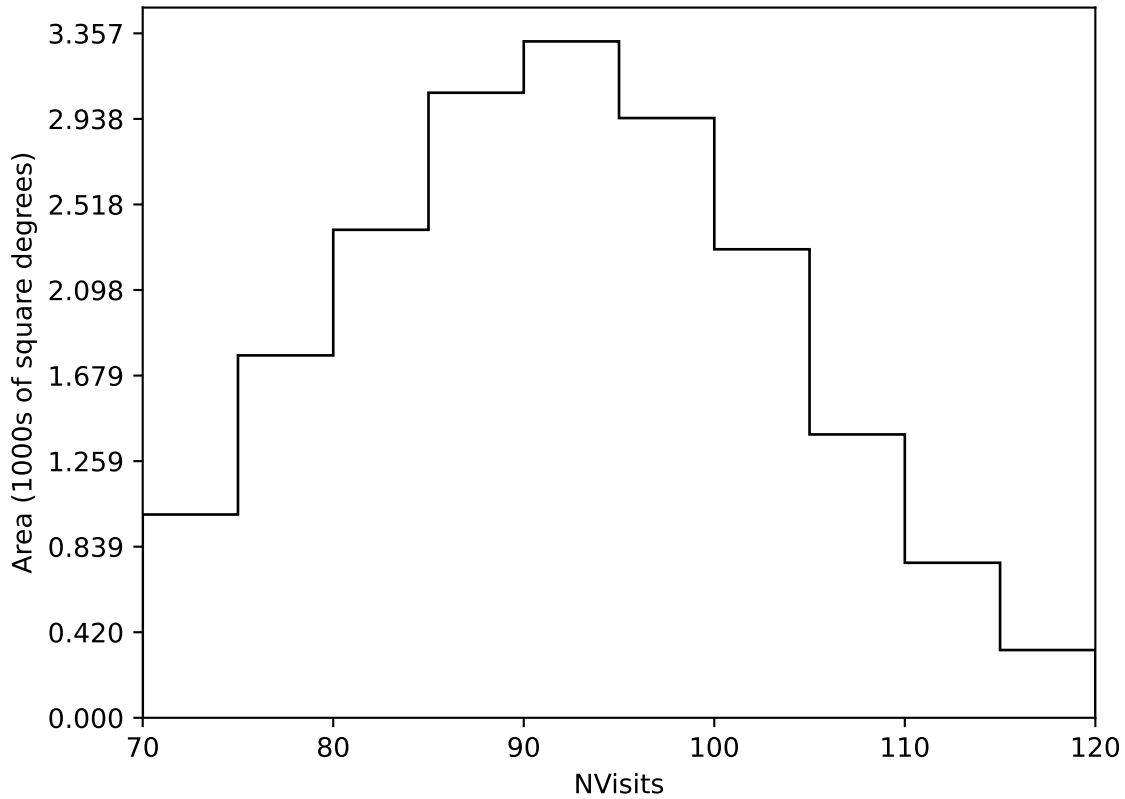
weather_cloudso0v3.4_10yrs Yr 1 all bands: NVisits
